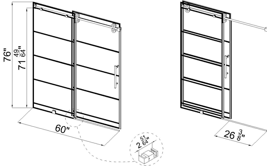
Wall to wall shower door
