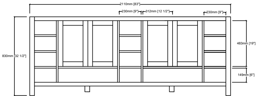
FRONT VIEW
