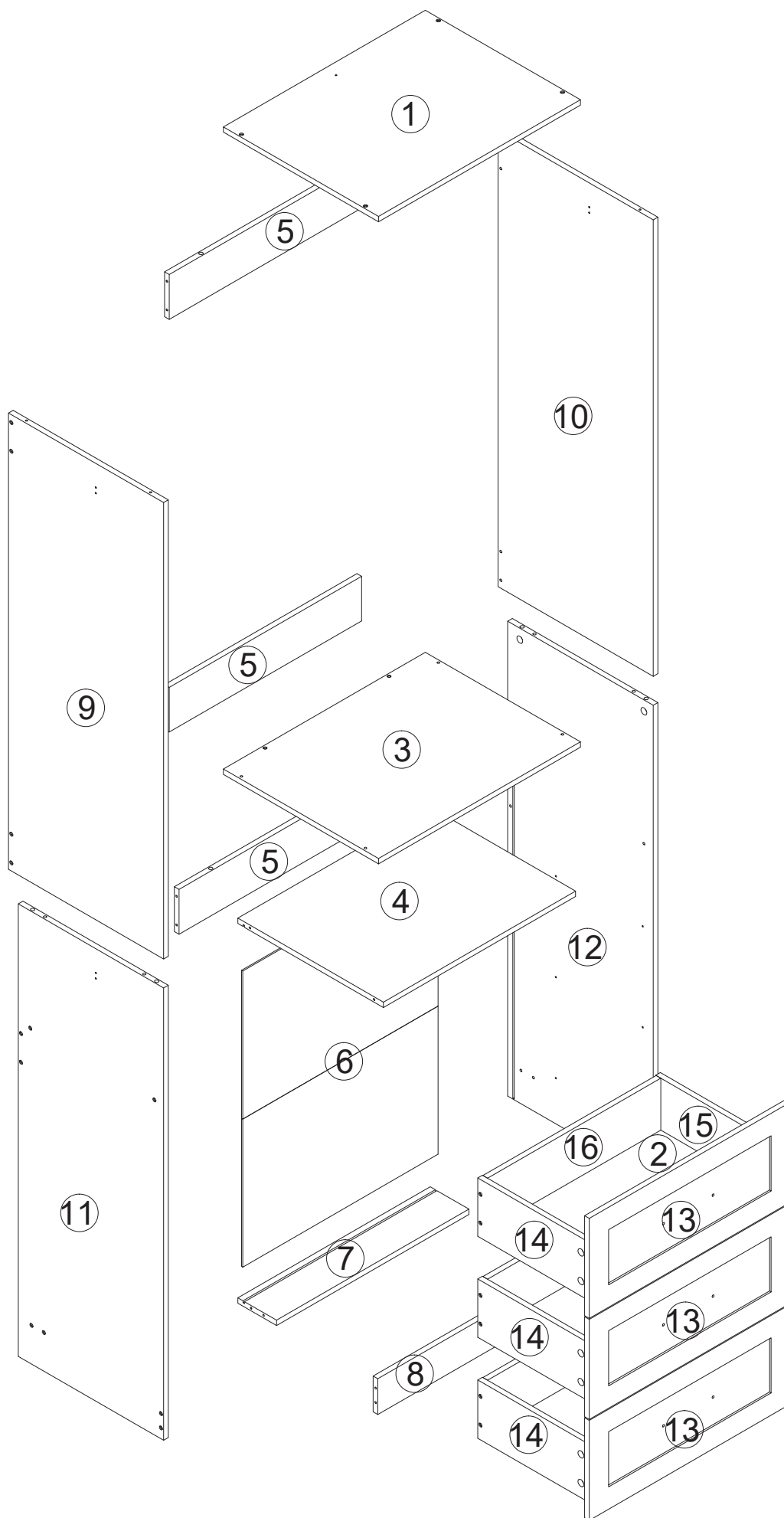
Explosive View
