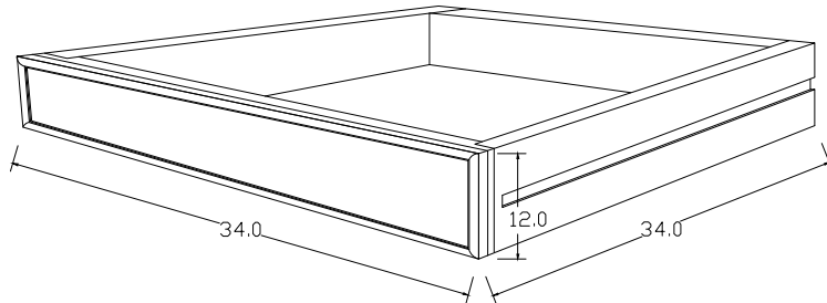
DETAIL DRAWER
