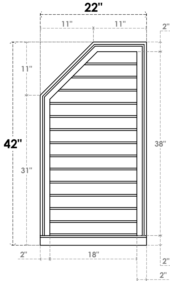
FRONT
