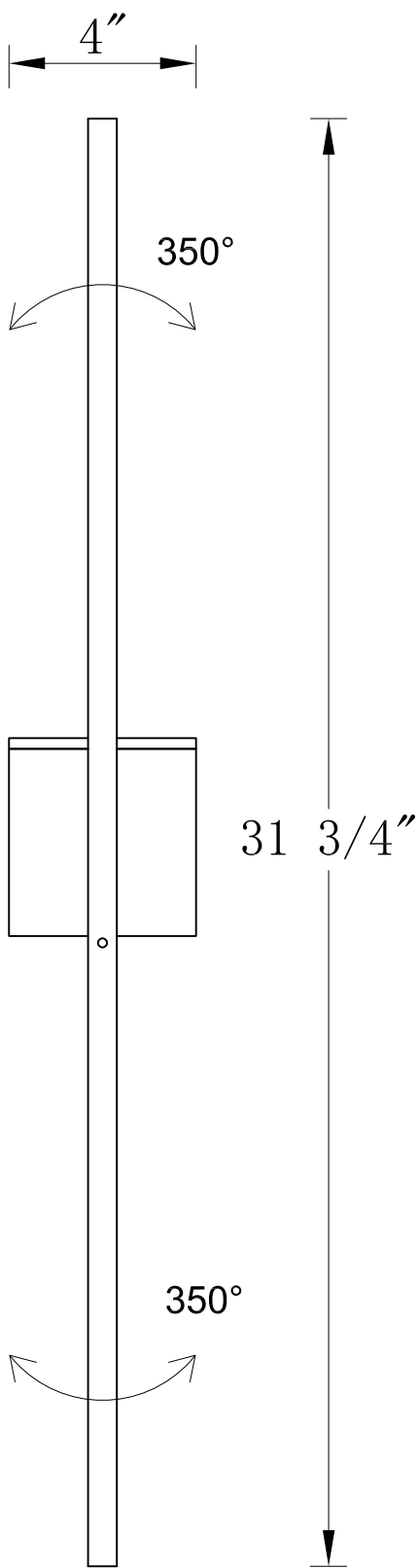
FRONT VIEW
