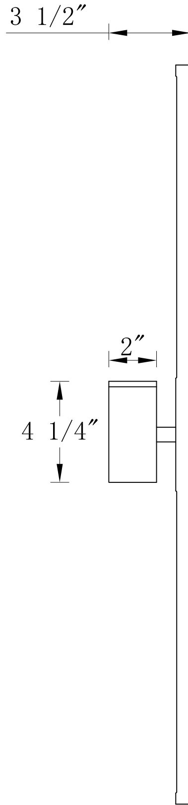
SIDE VIEW
