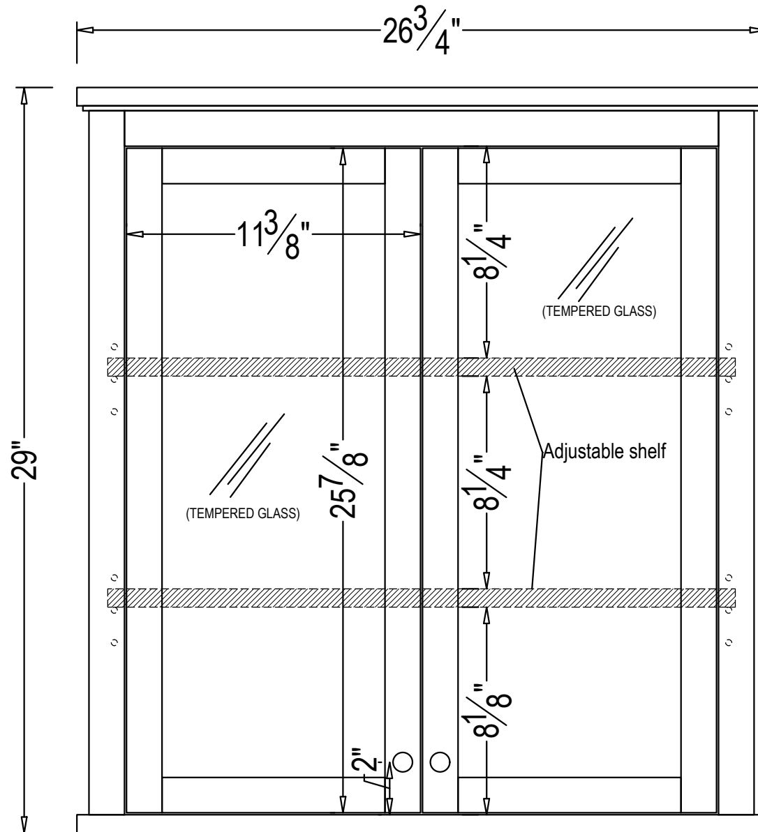
DORSET TOILET HUTCH W/GLASS
