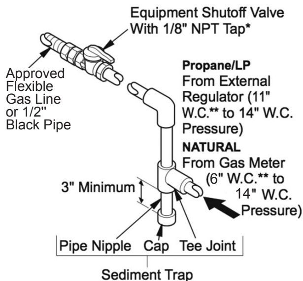
Fig. 10 - Gas Connection
