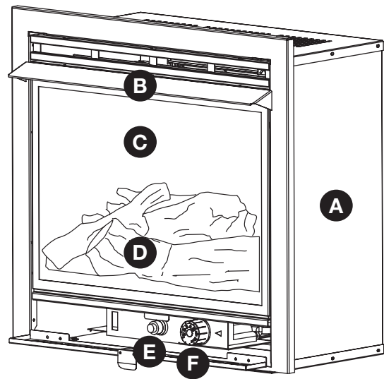
Fig. 1 - Vent-Free Dual Fuel Fireplace
