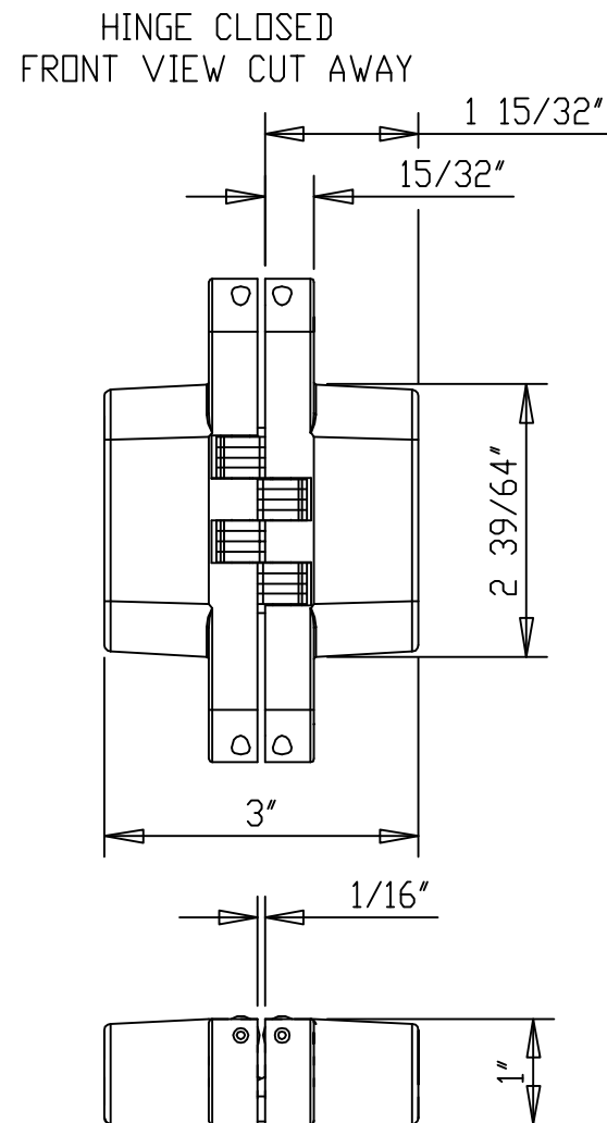
HINGE CLOSED TOP VIEW CUT AWAY
