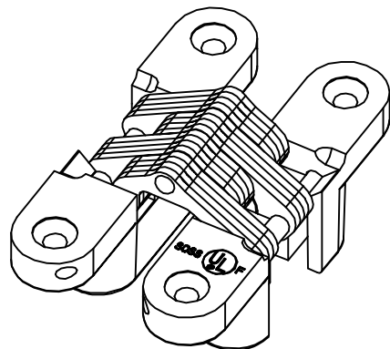
HINGE OPEN 180° ISOMETRIC VIEW
