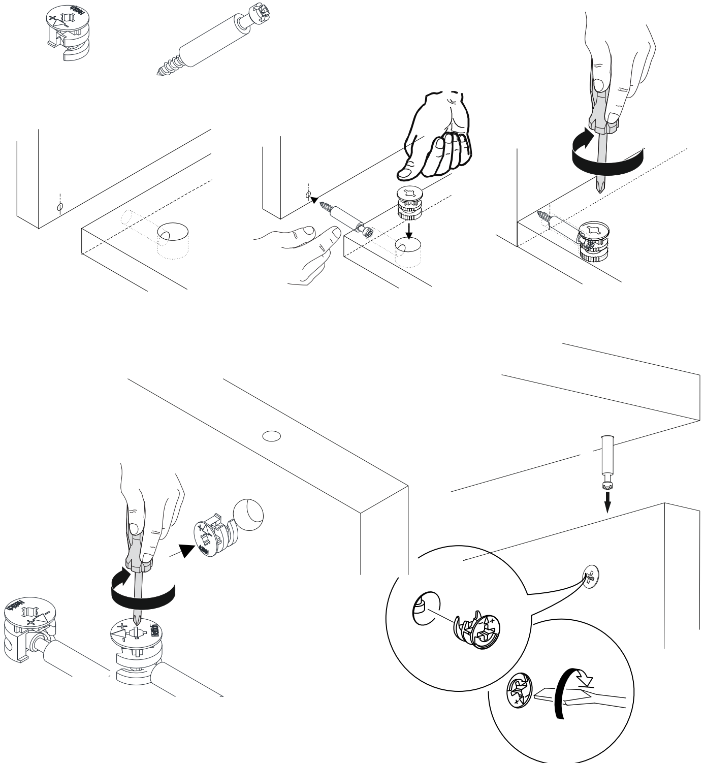
MINIFIX BODY
