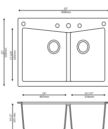
KGD-430B 33" x 22" x 9 1/2" Min Cabinet Size: 36" Drain Model #: BST-2 & ST-2
