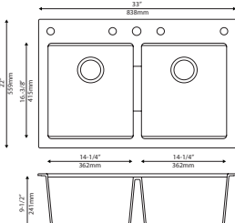
KGD-433B 33" x 22" x 9 1/2" Min Cabinet Size: 36" Drain Model #: BST-2 & ST-2
