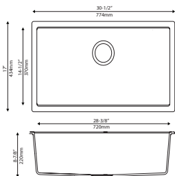
KGU-413B 30 1/2" x 17" x 8 7/8" Min Cabinet Size: 33" Drain Model #: BST-2 & ST-2
