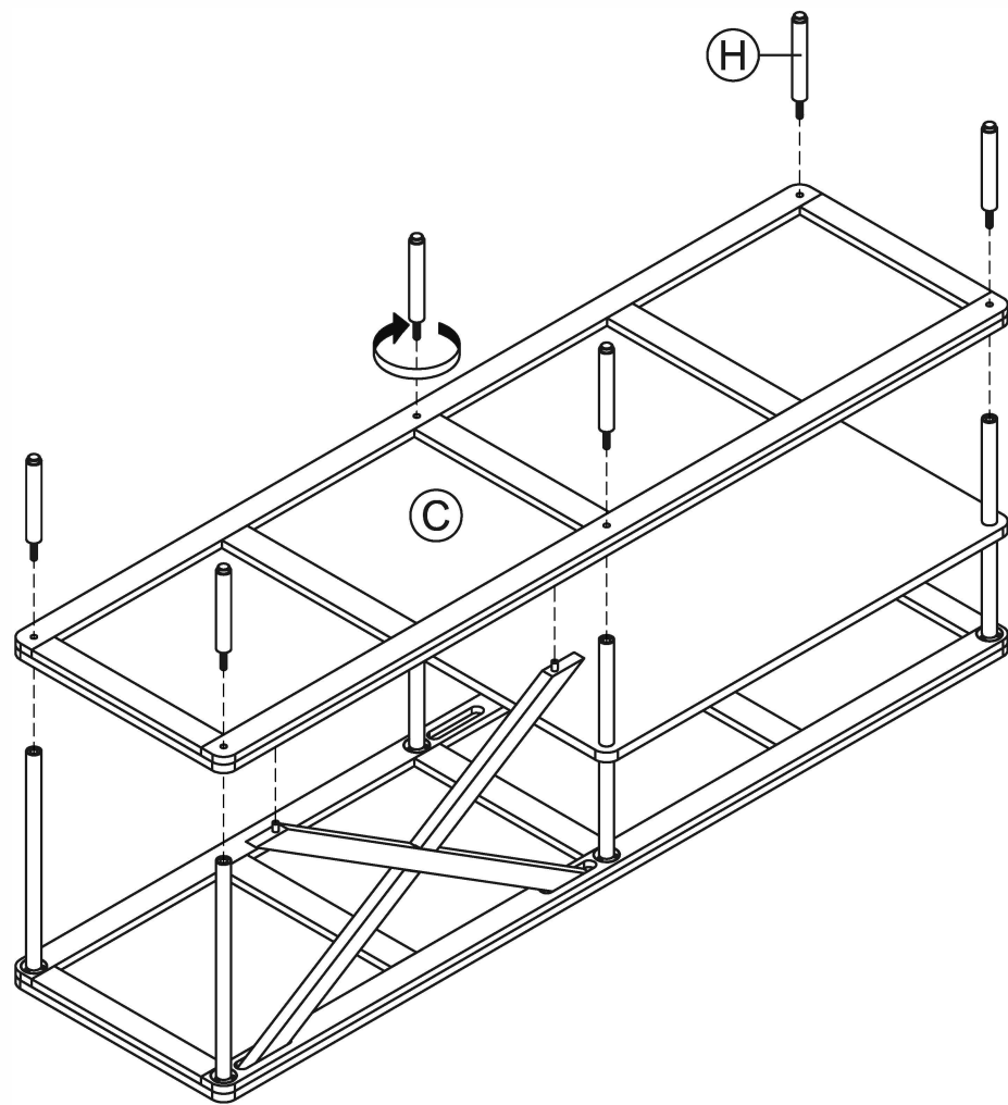
STEP 3 ATTACH BOTTOM PANEL AND LEG TO UNIT.
