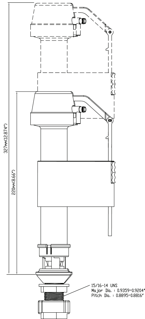
K830-11BX ADJ BALLCOCK
