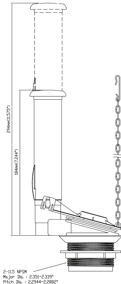
K830-16BX-1 ADJ FLUSH VALVE
