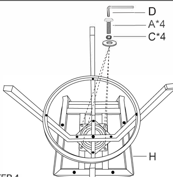
STEP 4. Secure the seat cushion (H) to the swivel plate (G) using screws (A*4) and washers (C*4).
