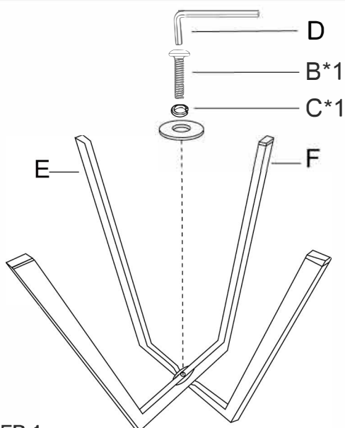
STEP 1. Secure leg (E) and leg (F) with screw (B*1) and washers (C*1).
