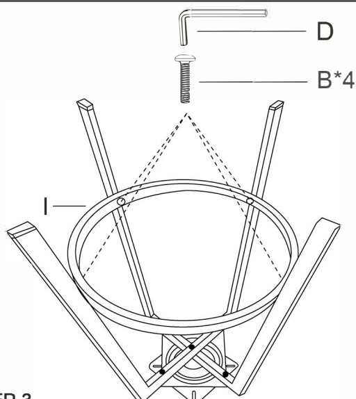
STEP 3. Secure the footrest (I) to the chair legs (E & F) using screws (B*4).
