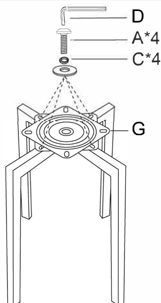
STEP 2. Secure the swivel plate (G) to the chair legs (E & F) using screws (A*4) and washers (C*4).
