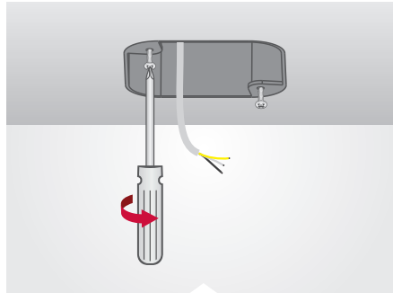
STEP 2: 1. For 3" & 4" Jbox, install 2 long screws (provided) to Jbox leaving minimum 1/2" space to ceiling. 2. For 2.75" Jbox, Do Not install screws until later, Step 5.
