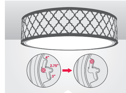
STEP 5: 1. For 3" & 4" Jbox, align the holes on the base of the fixture with the pre-installed screws from the Jbox using the proper slots as indicated in the above diagram. 2. For 2.75" Jbox, install base of the fixture to the Jbox by attaching 2 screws (provided) as shown in the diagram.
