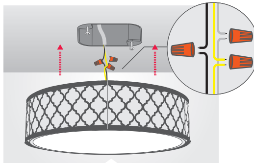
STEP 4: Make ground connection. Attach black AC wire from fixture to black AC wire from Jbox. Connect white wire from fixture to white wire from Jbox.
