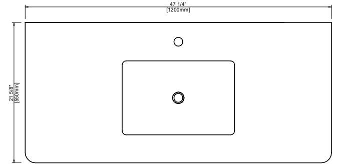
COUNTERTOP PLAN VIEW
