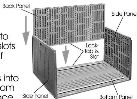
Bottom Panel
