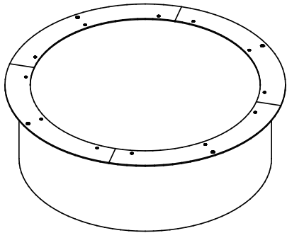
LEG (Ø450x165mm)
