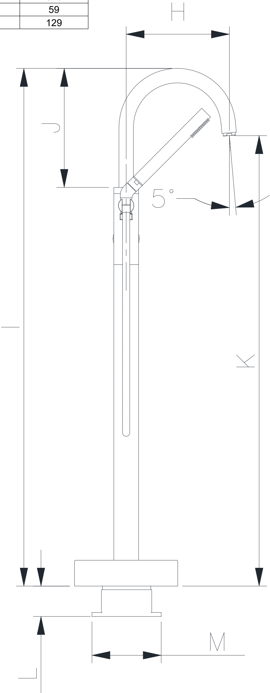
SIDE VIEW OF FAUCET
