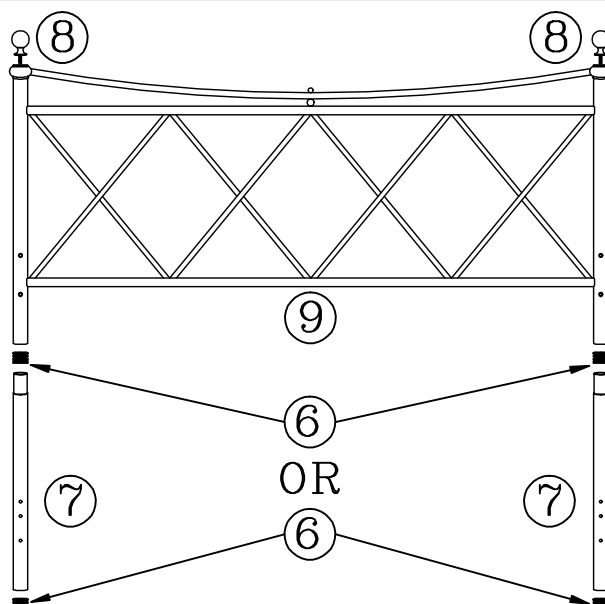
FOOTBOARD ASSEMBLY
