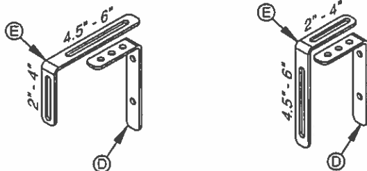
Optional Mountings
