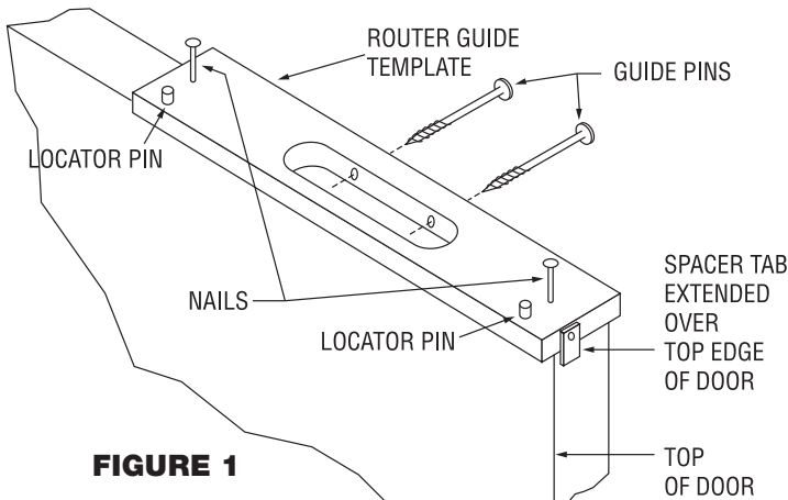
FIGURE 1 References the various components of the hinge router guide template. Become familiar with this terminology as it will be used throughout these instructions.
