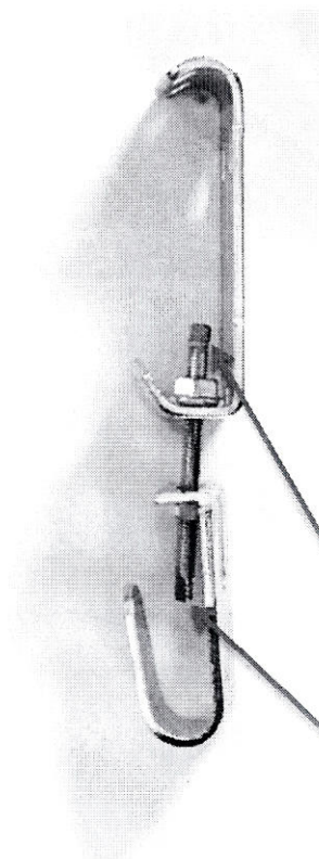
Figure 2: Adjustable J-hook side profile, showing the double crimped ends of the threaded rod.
