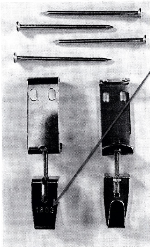
Figure 1: Standard adjustable j-hook pack. The number 1803 is the manufacturer's series number for production
