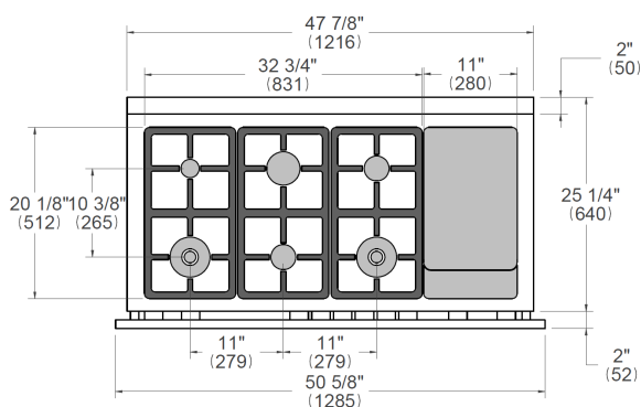
WORKTOP DETAILS
