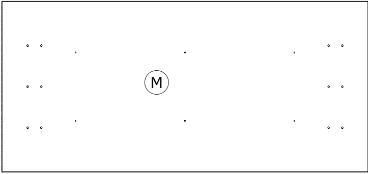
CA3741 1715x800x30mm
