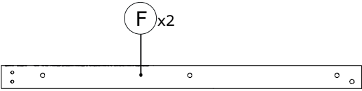
FS4244 1254x80x30mm
