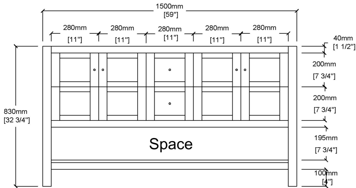
FRONT VIEW
