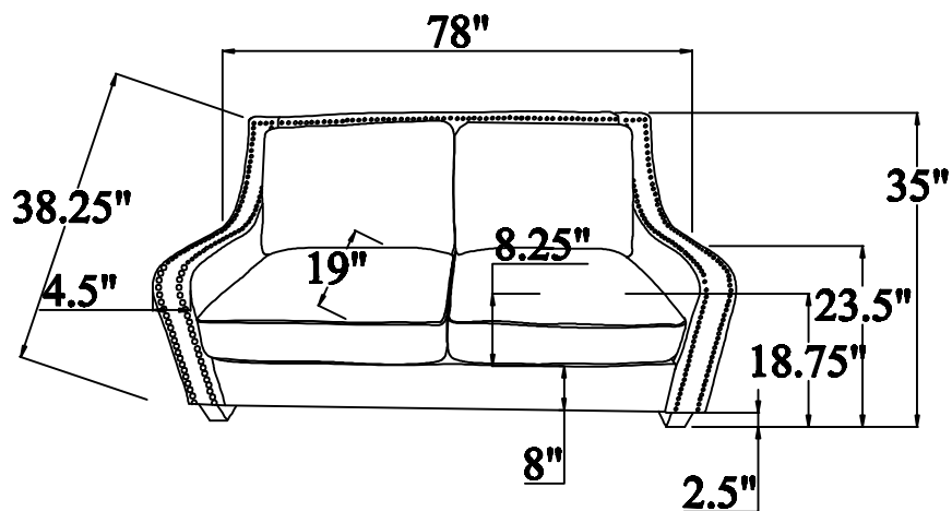
SOFA : L78"*D38.25"*H35"
