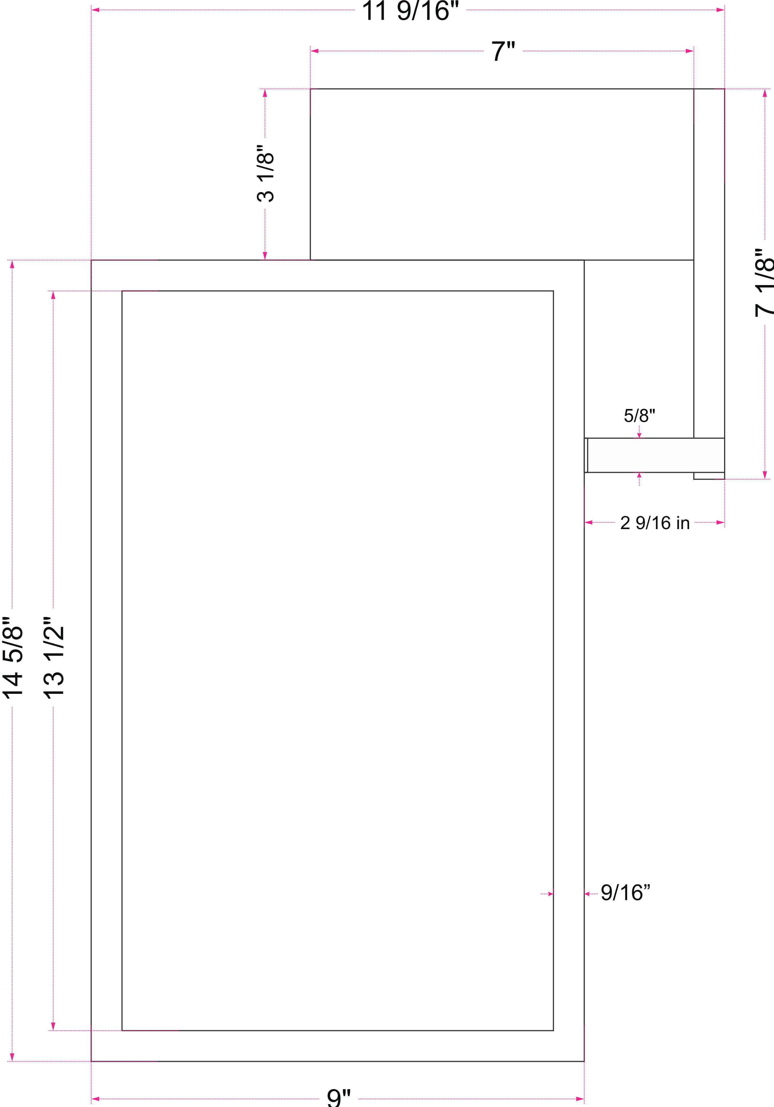
Side View
