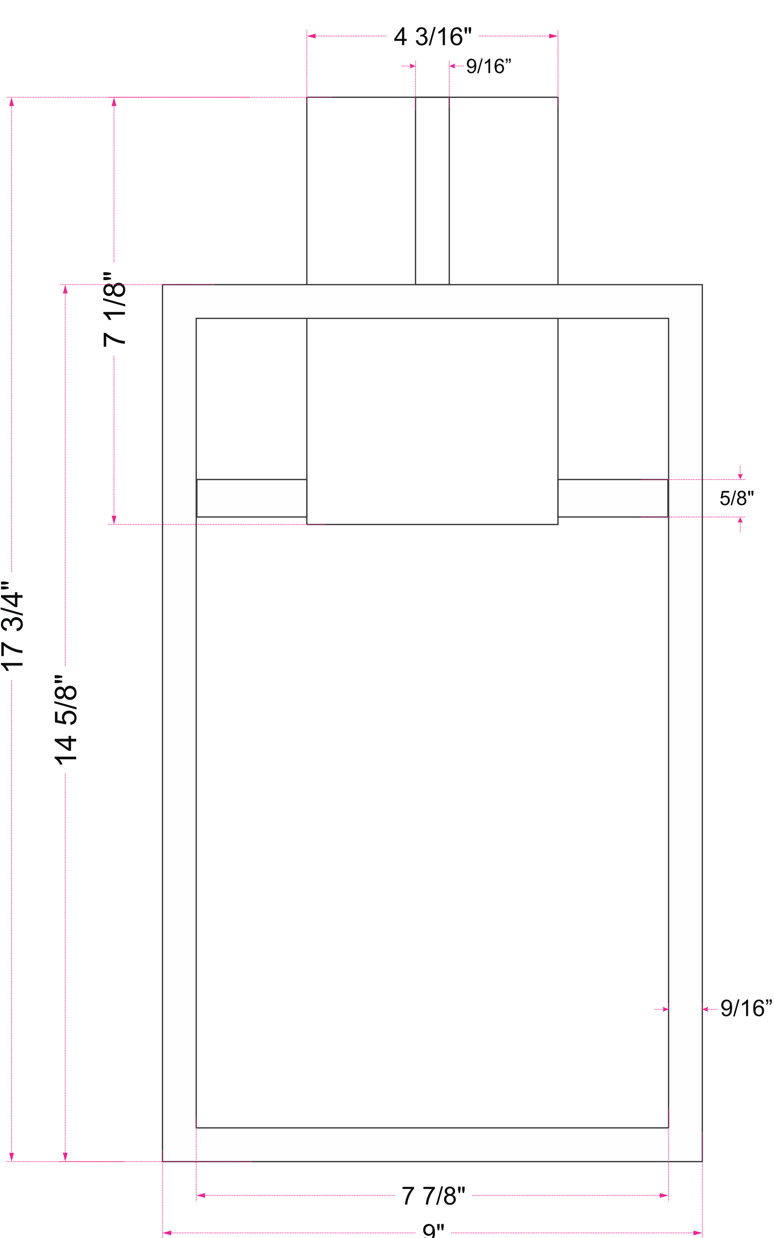
Front View
