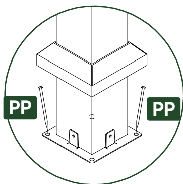
Soft foundation
