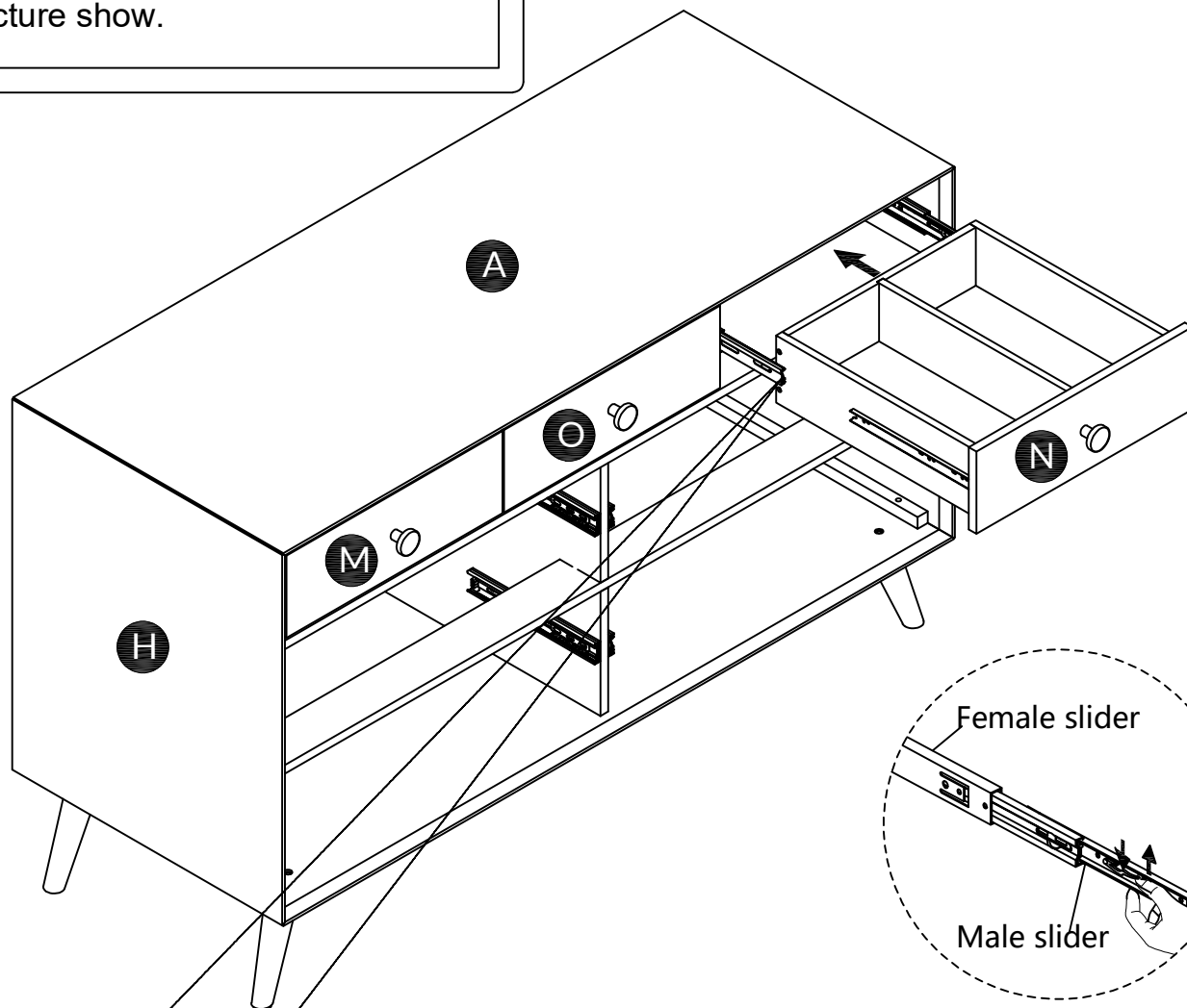
Schematic diagram of slide rail disassembly
