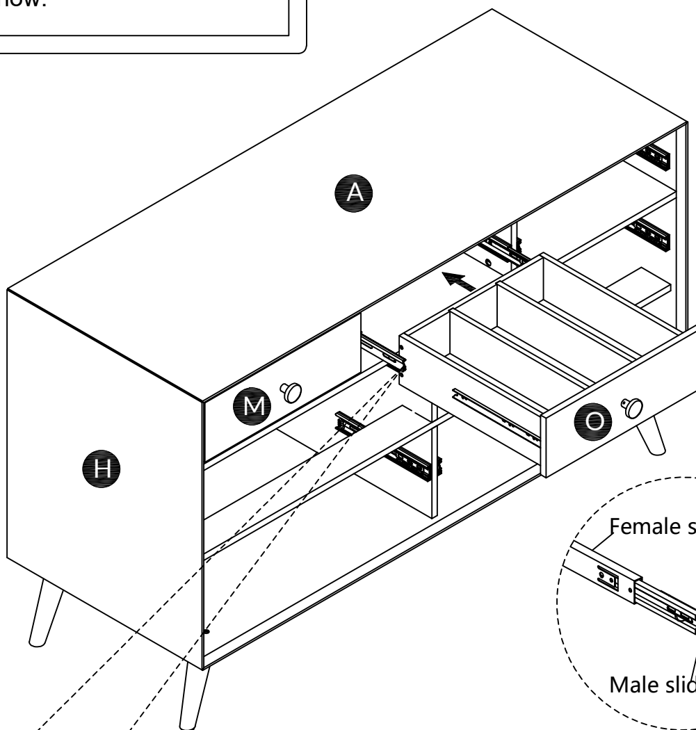
Schematic diagram of slide rail disassembly
