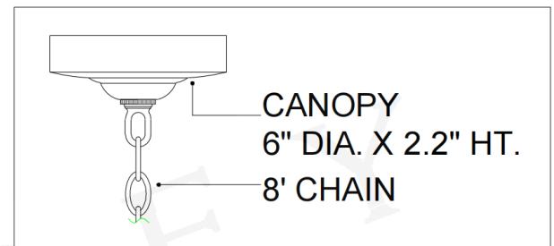
CANOPY DETAIL
