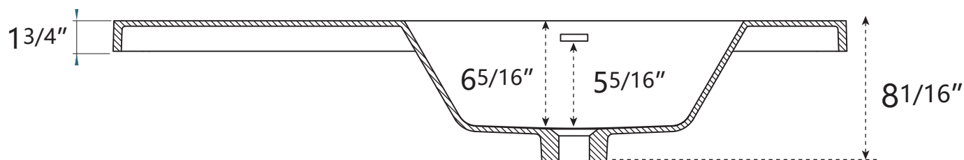
FRONT VIEW
