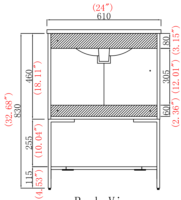
Back View
