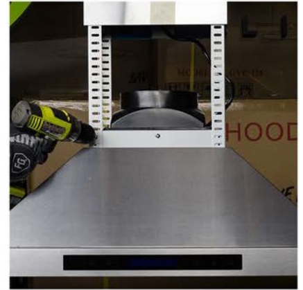
20. Feed the power cord through the ceiling hole.
