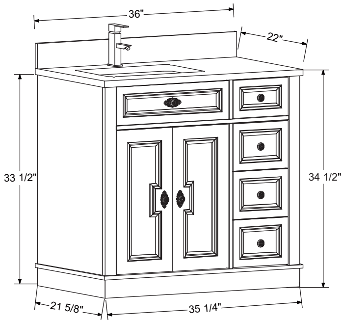
Vanity Front
