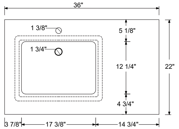
Sink
