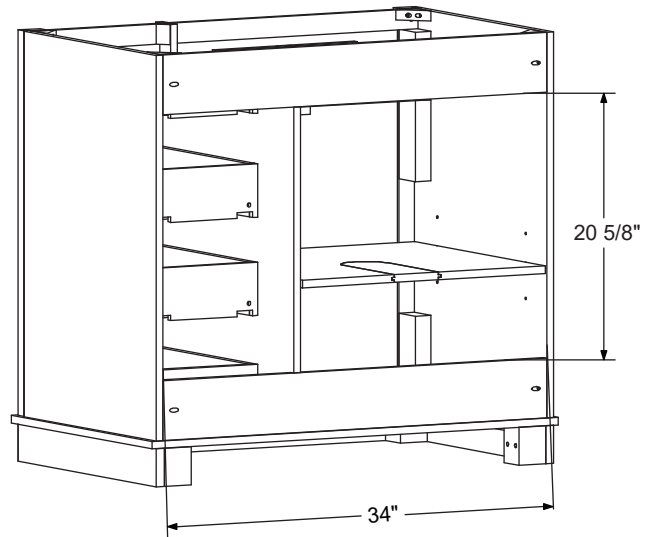
Vanity Back
