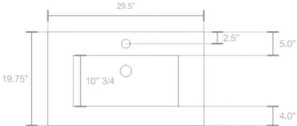
SINK CUT OUT OPENING 400 (15.75"W) x 273 (10.75"D)
