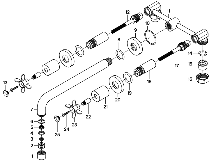
Hot Cartridge: No.12- KSRPL8000C
