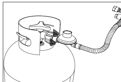
Regulator/Cylinder Connection
