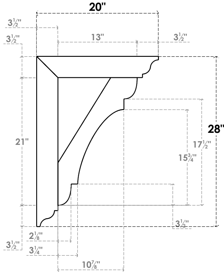
SIDE PROFILE
