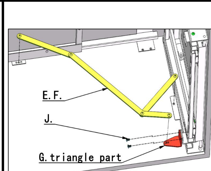
Step 5: Connect "E, F & G" with "G" & "J" as shown
