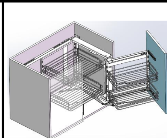
Step 7: Put 2 pcs big baskets "M" and 2pcs small basket "N" and Done!
