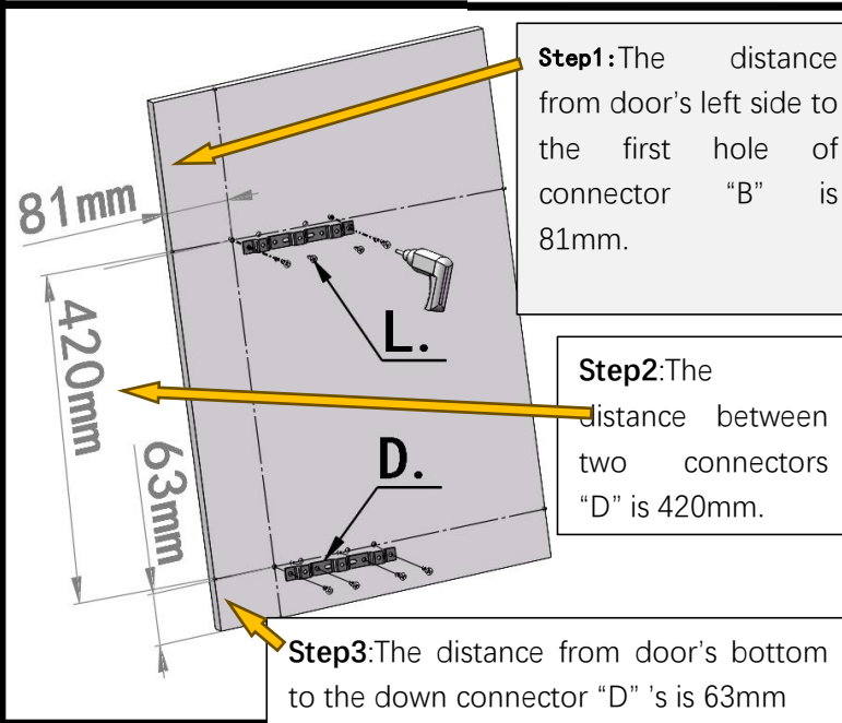
Step 5: Fix the 2pcs "D" on the door panel as show.
