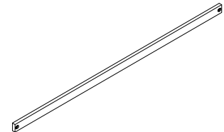
16 (1555x50x15mm) x 1
