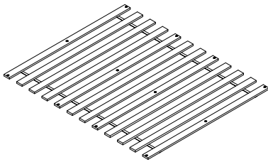
17 (1555x50x15mm) x 12
