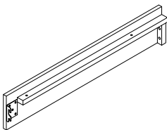
13 (1041.5x197x57mm) x 2
