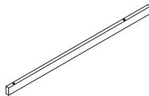
18 (926.5x45x25mm) x 1
