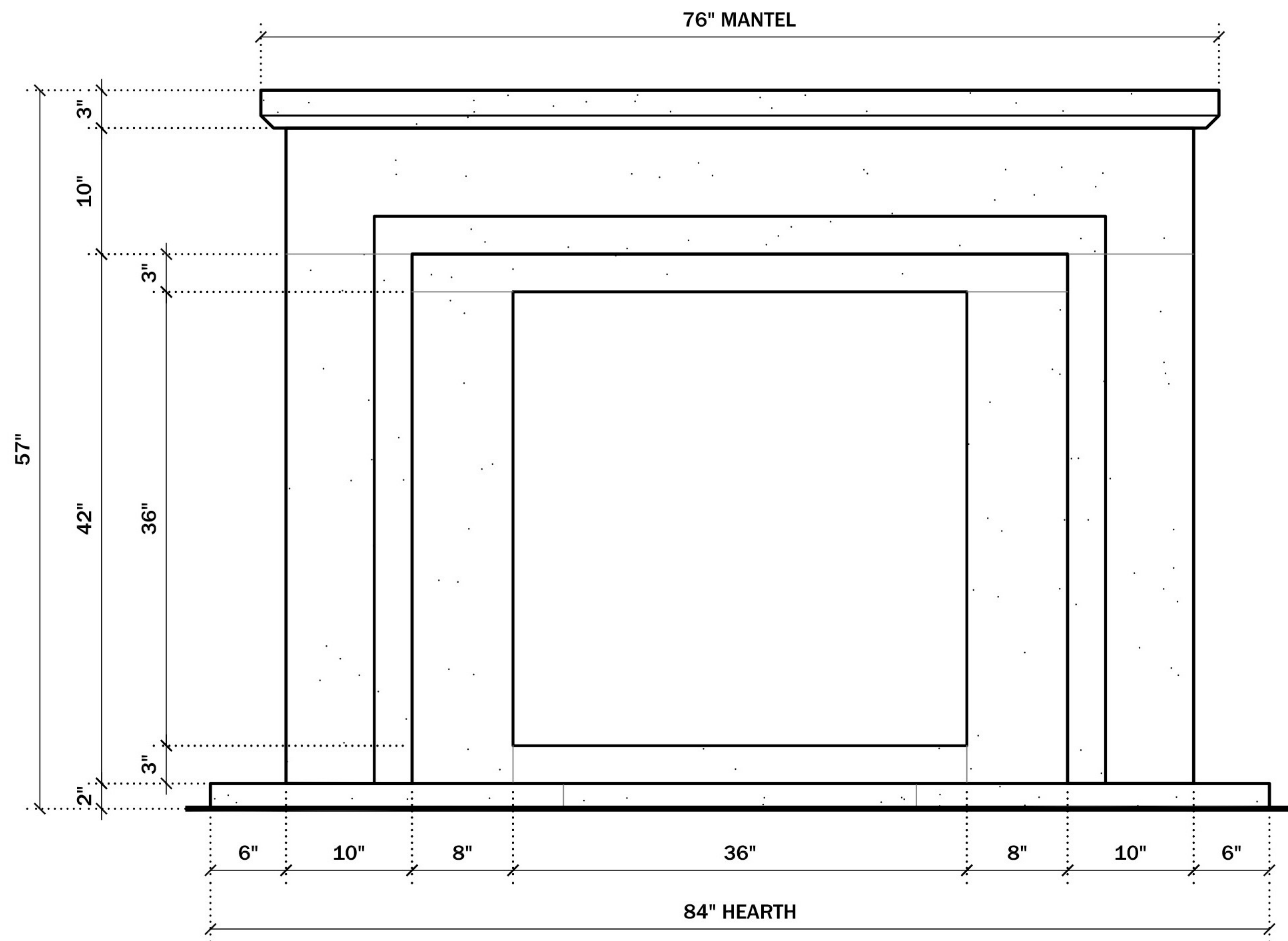
FRONT ELEVATION
