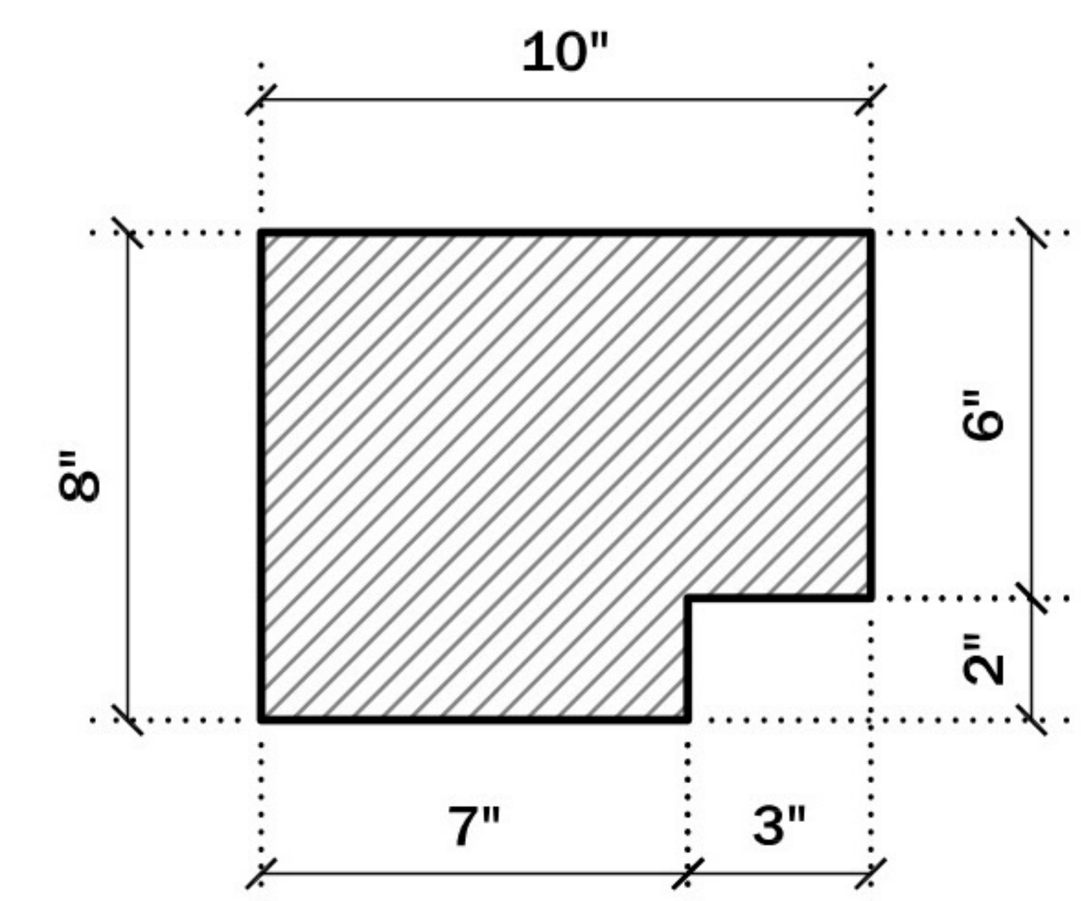
LEGS PROFILE
