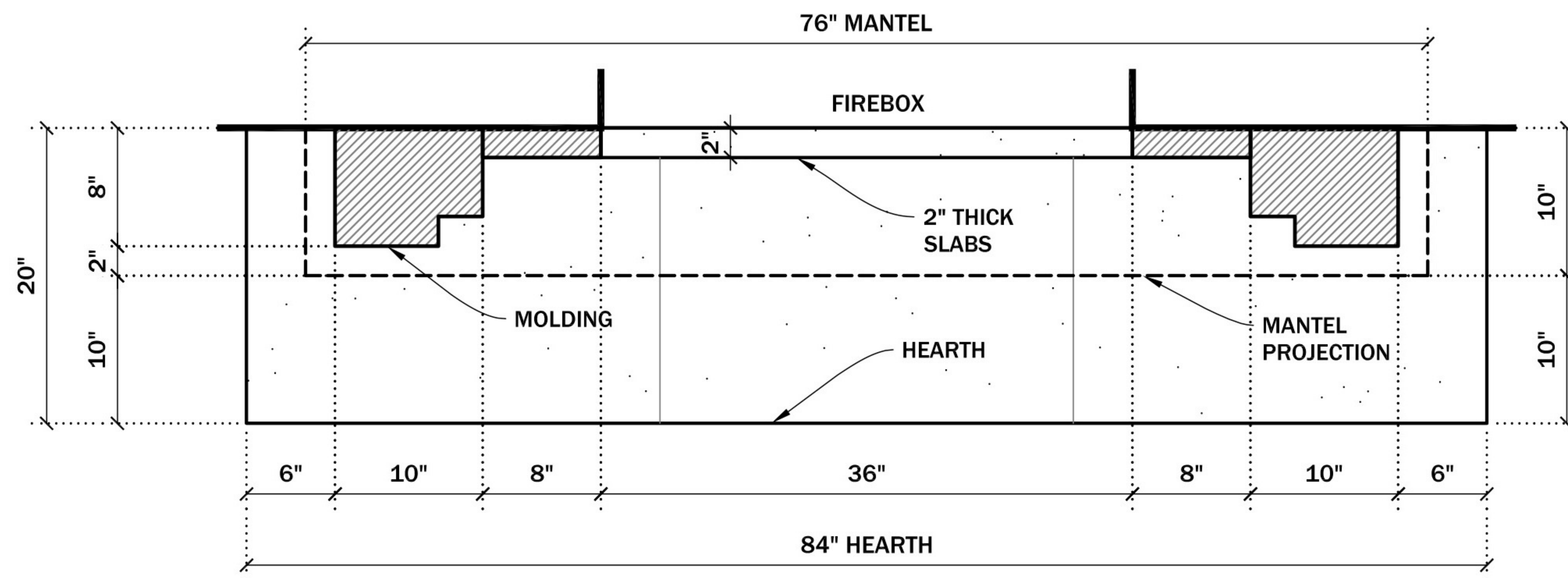
PLAN VIEW
