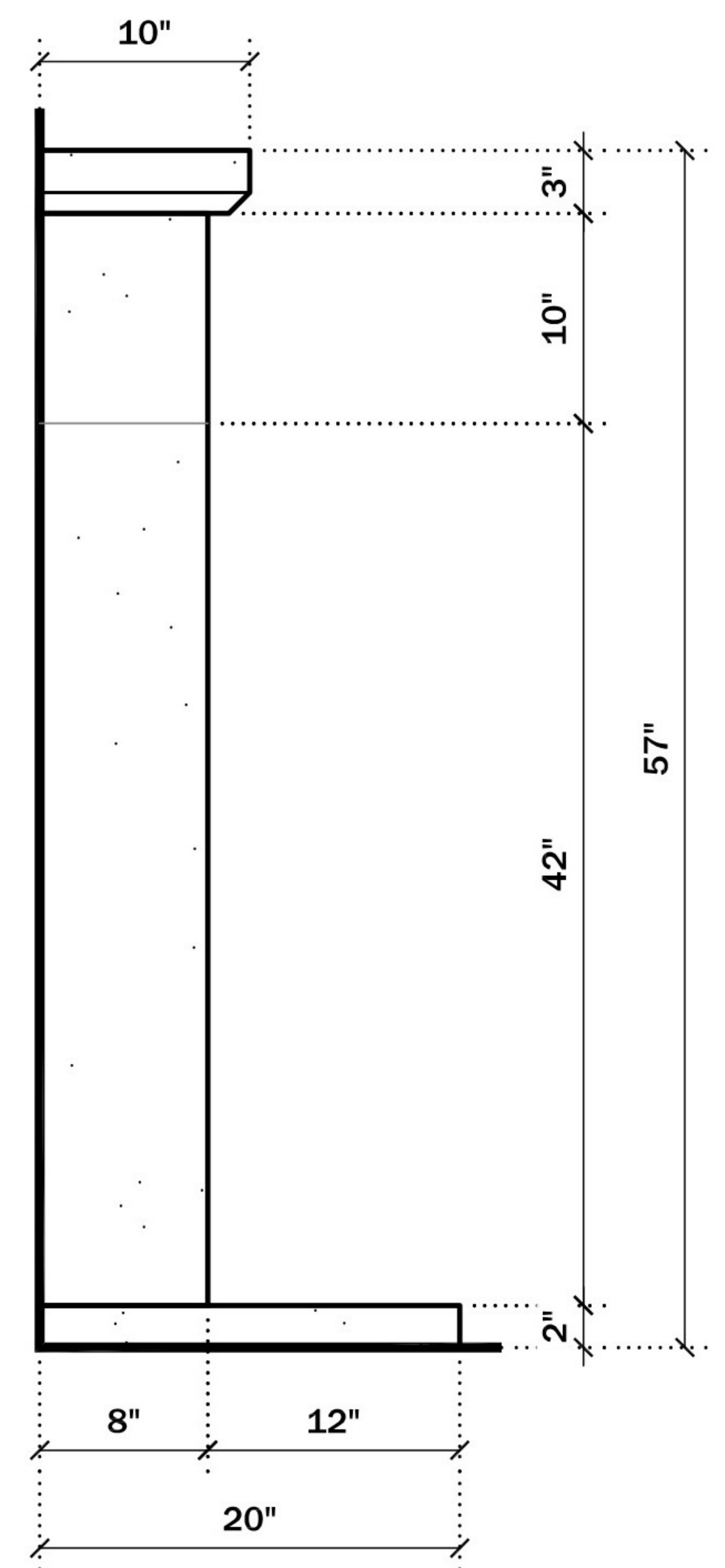
SIDE VIEW
