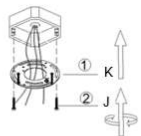
OUTLET BOX
