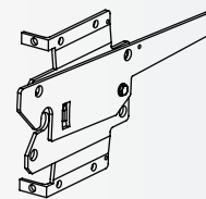
Latch Catch (1) with 1 1/4" Black Stainless Steel Screws (6)
