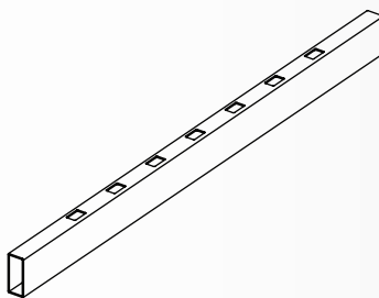
Top Rail (1) 1 1/2" x 3 1/2" x 47 3/4"
