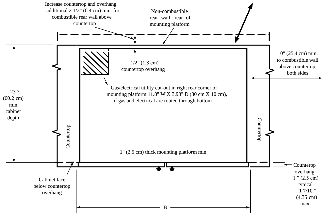
Gas connection and power cord may be routed through bottom or back of chassis
