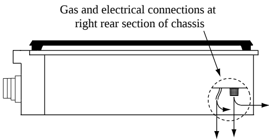
Gas connection and power cord may be routed through bottom or back of chassis
