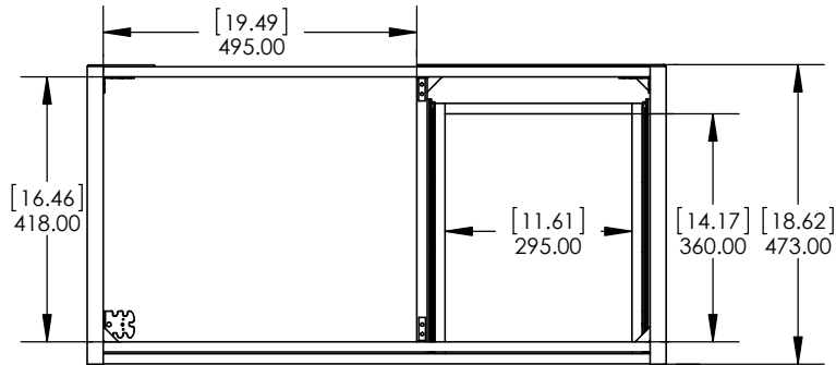
Top View / Vista Superior
