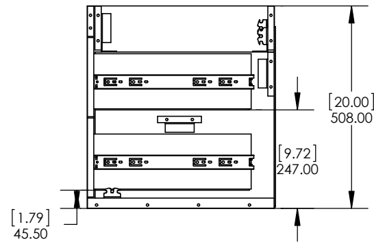
Side View / Vista Lateral
