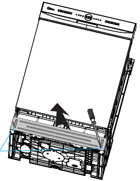
Kick Plate Screws (2)
