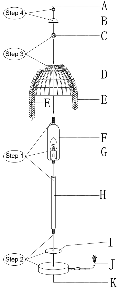
Lighting structure explosion diagram
