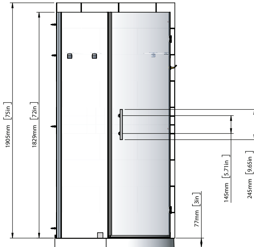
Front View - Vue de face - Vista frontal
