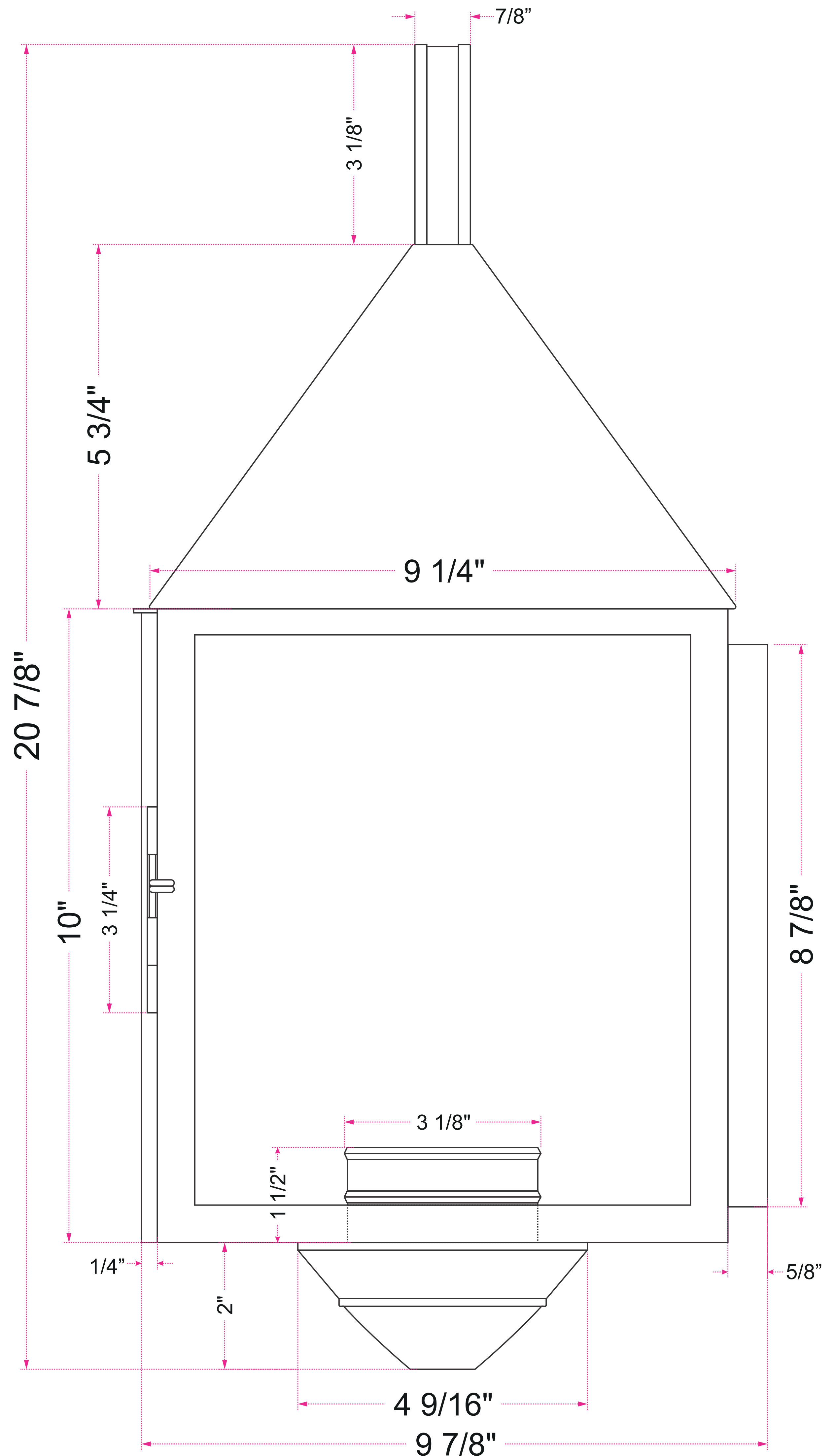
Side View
